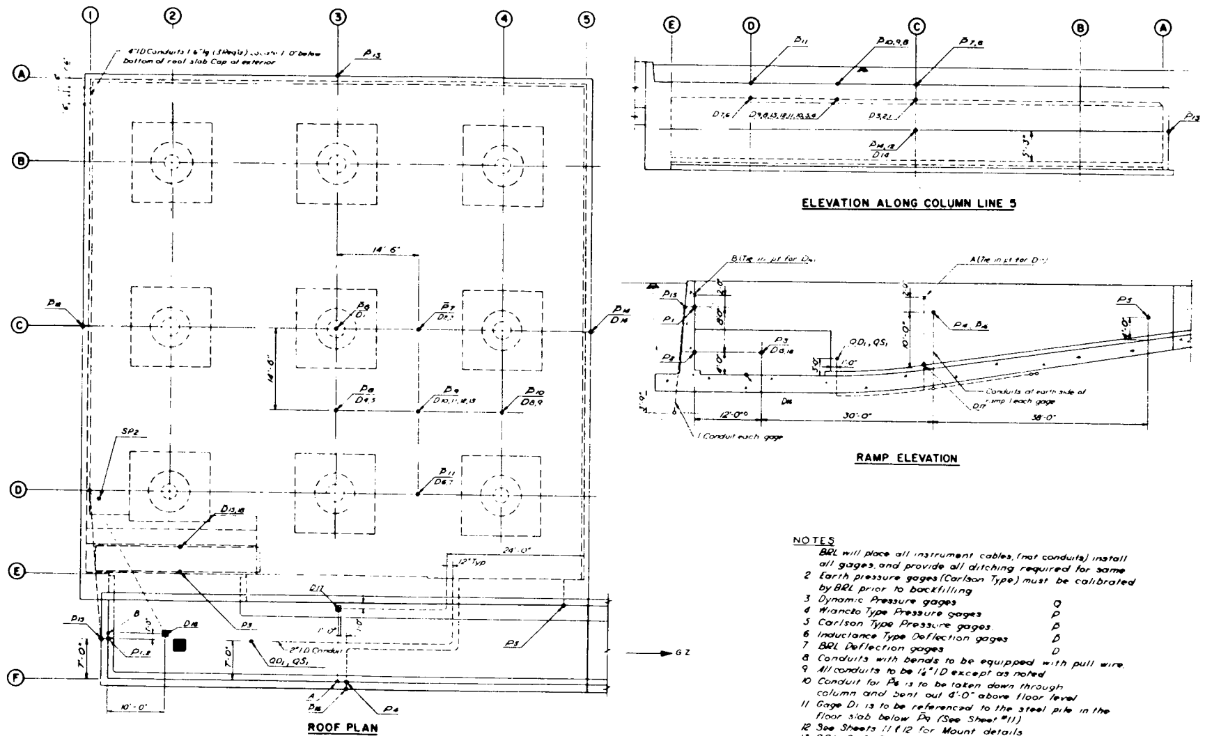
Fig. 6—Instrumentation layout.
